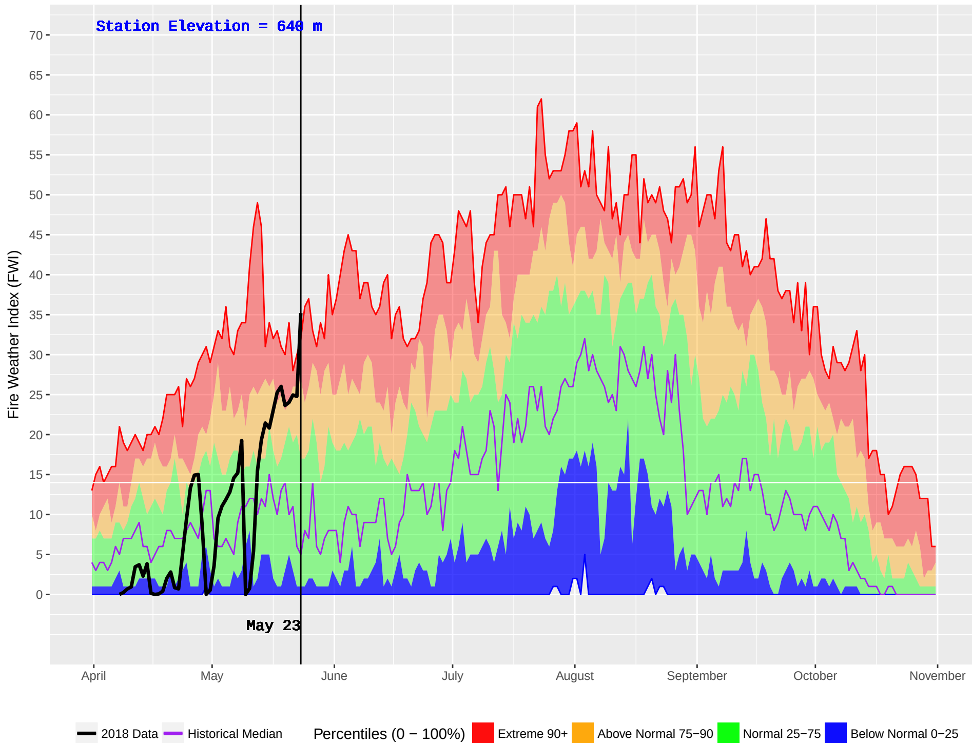
TURTLE (286) : Historical (1977–2016) and Current (2018) Noon Fire Weather Index (FWI)
