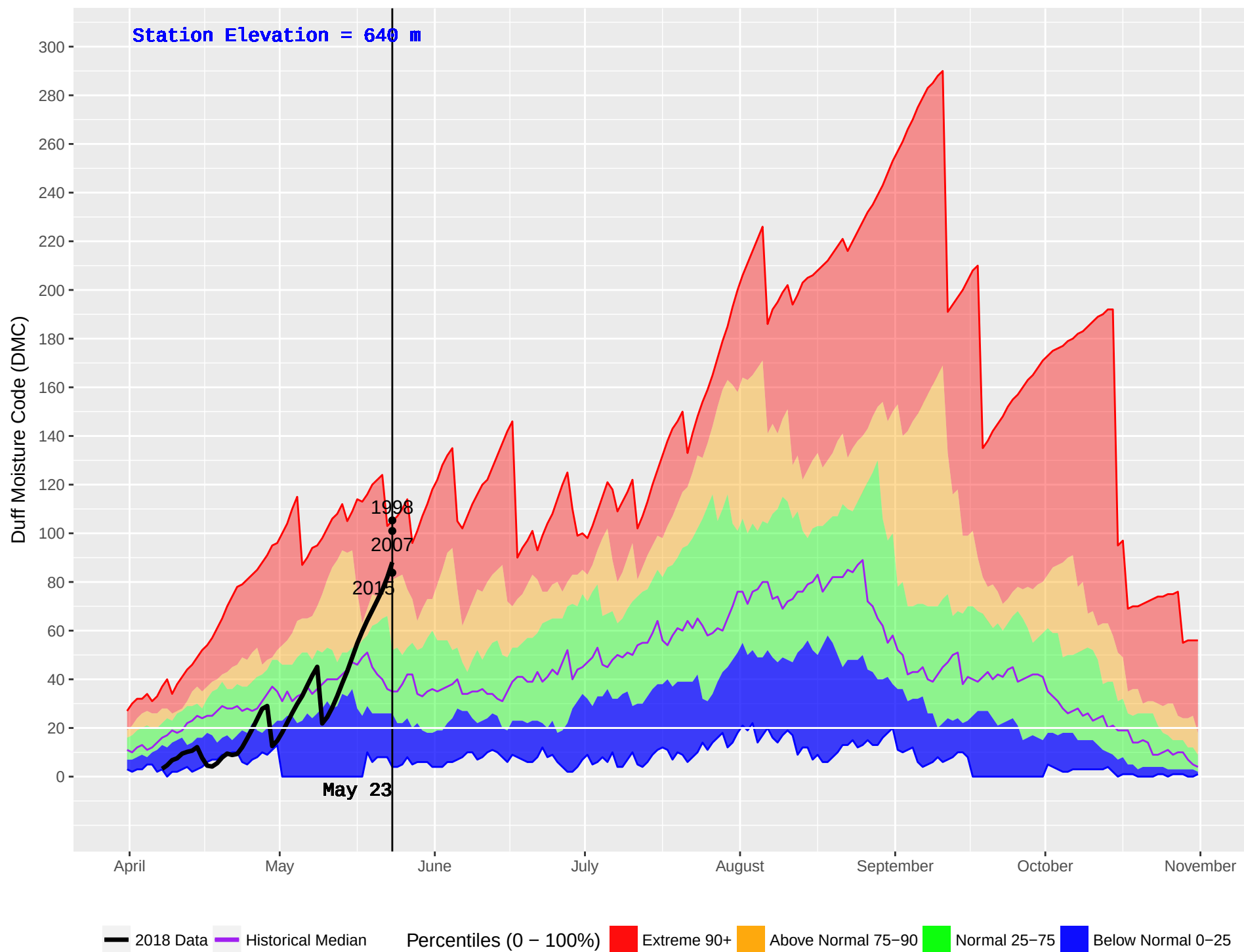
TURTLE (286) : Historical (1977–2016) and Current (2018) Noon Duff Moisture Code (DMC)
